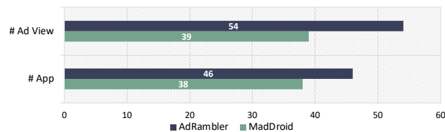
Figure 7: Comparison with the state-of-the-art approach.
